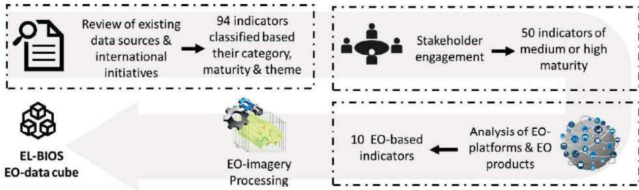
Figure 1 Methodology outline
